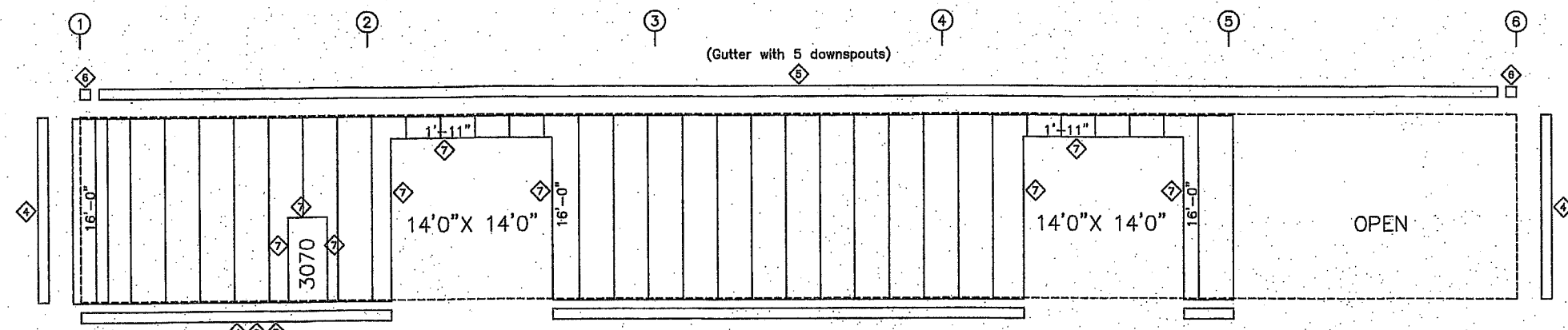
SIDEWALL SHEETING & TRIM: FRAME LINE A PANELS: 26 Ga. PBR - Ash Gray
