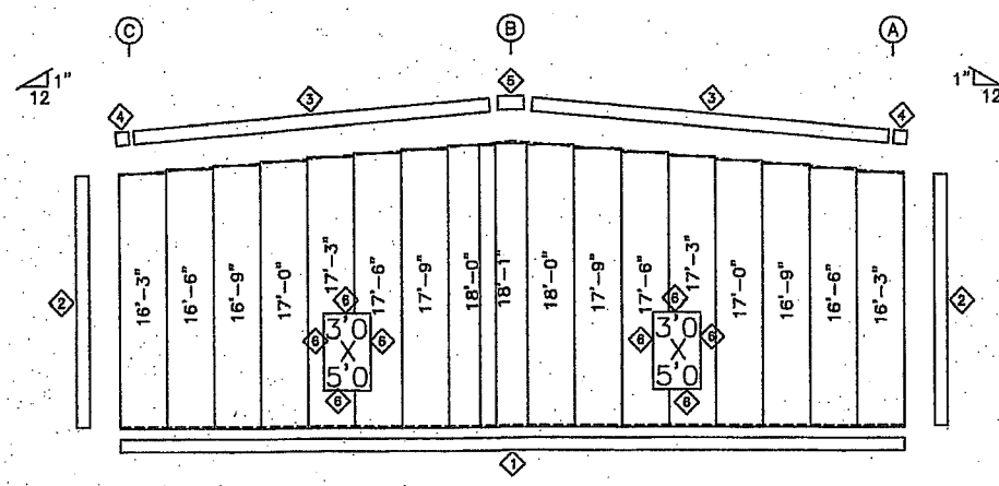
ENDWALL SHEETING & TRIM: FRAME LINE 1 PANELS: 26 Ga. PBR - Ash Gray
