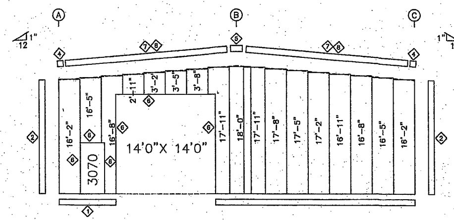
ENDWALL SHEETING & TRIM: FRAME LINE 5 PANELS: 26 Ga. PBR - Ash Gray
